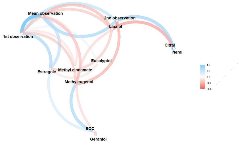
Figure 5. Network correlation plot (NCP) among observations and main essential oil components
